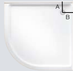
CARRA Shower Base - Rear Waste 1000 x 1000mm only A: 150mm B: 150mm
