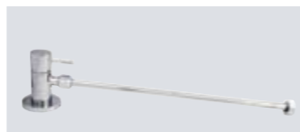
PROGETTO DELUXE ANGLE VALVE AND RISER SET | 26901 | $45 • Soft copper riser (easy to bend) • Includes 10 & 15mm connections
