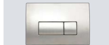
SPEEDO PNEUMATIC FLUSH PANEL METAL POLISHED STAINLESS STEEL | P100MPS | $269 BRUSHED STAINLESS STEEL | P100MBS | $319 • 210W x 140H x 15D • Top, front or remote mounted (up to 3 metres from cistern)
